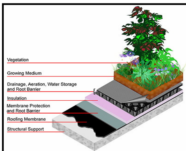
Figure 1: Green roof components
