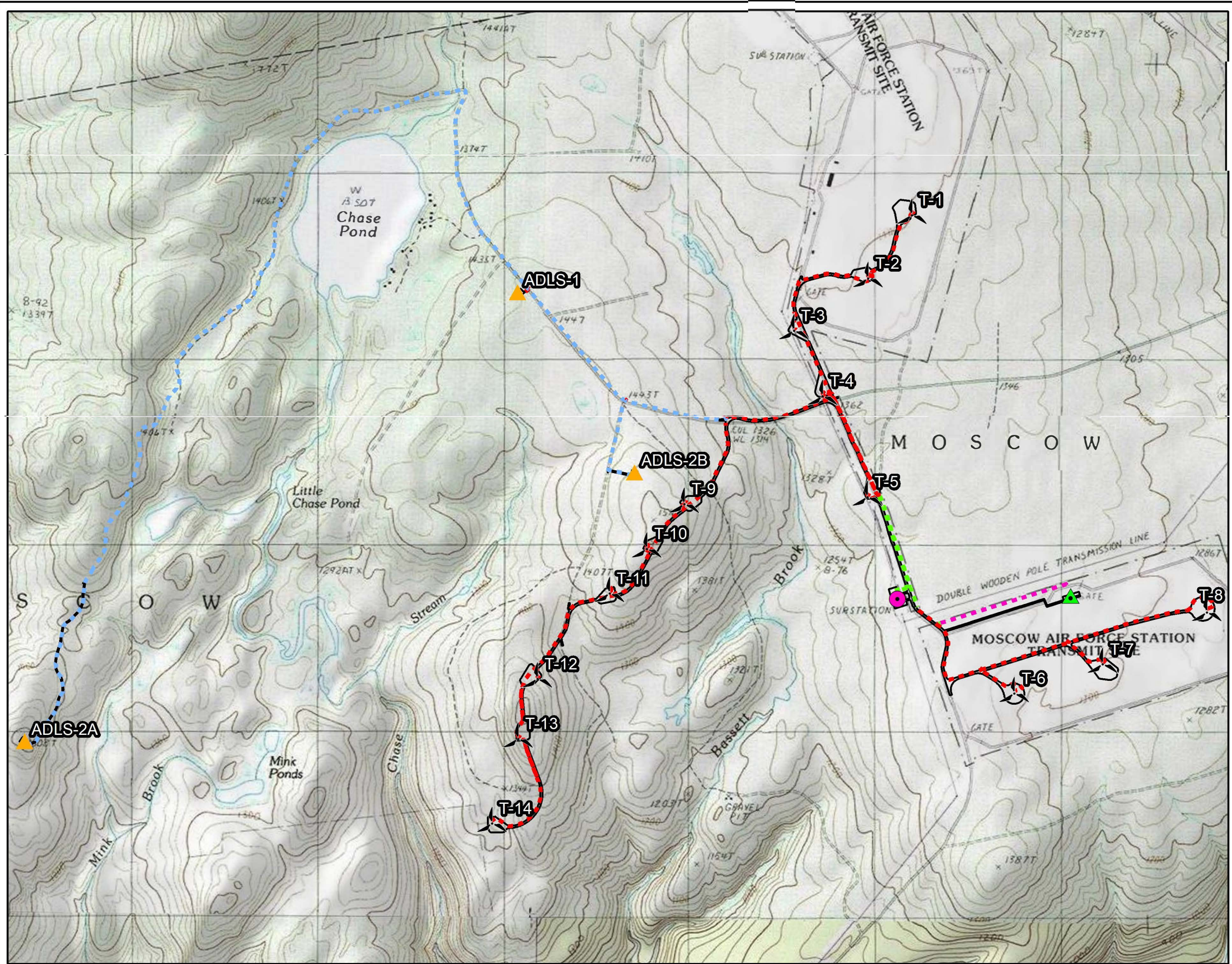
Figure 3-1 Project Layout and Location Western Maine Renewable Energy Project
